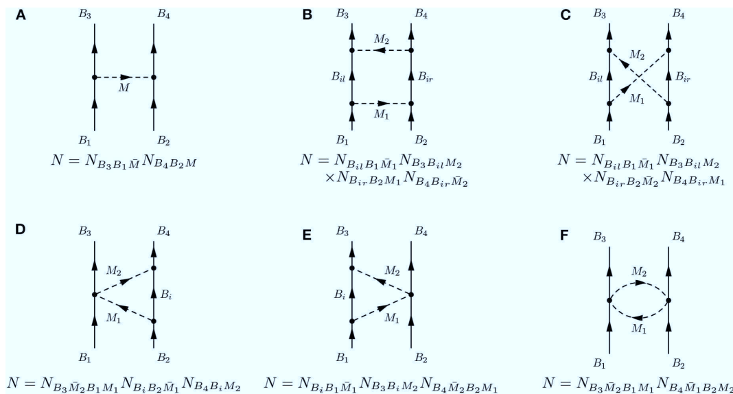
FIGURE 7 | One- and two-meson-exchange contributions and corresponding SU(3) factors. (A) One-meson exchange, (B) planar box, (C) crossed box, (D) left triangle, (E) right triangle, and (F) football diagram.
