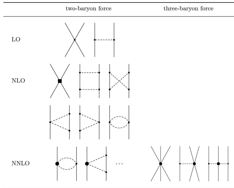
FIGURE 5 | Hierarchy of baryonic forces. Solid lines are baryons, dashed lines are pseudoscalar mesons. Solid dots, filled circles, and squares denote vertices with \Delta_i = 0, 1, and 2 , respectively.
