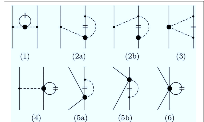
FIGURE 12 | Effective two-baryon interaction from genuine three-baryon forces. Contributions arise from two-pion exchange (1), (2a), (2b), (3), one-pion exchange (4), (5a), (5b), and the contact interaction (6).
