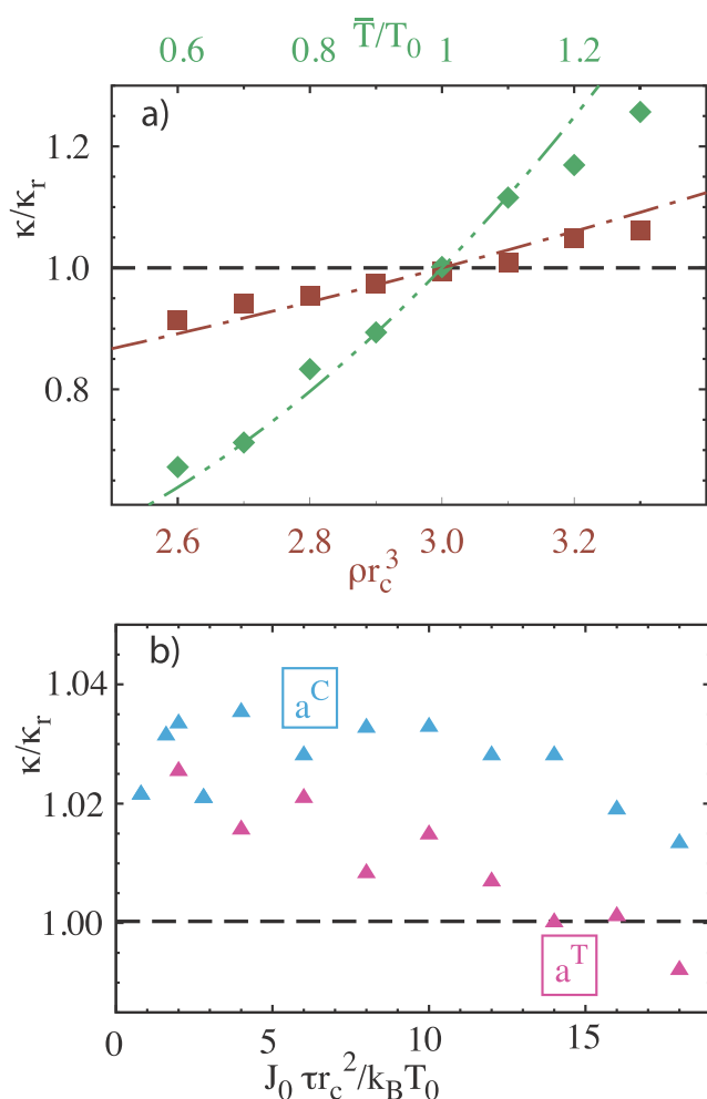
FIG. 4. (a) Normalized heat-conduction coefficient \kappa/\kappa_T as a function of temperature and density for relatively weak thermal gradients ( \Delta T/T_0 \lesssim 0.05 ). The normalizing factor \kappa_T = 146 k_B / (\tau r_c) is calculated for the reference values \bar{\rho} = 3/r_c^3 and \bar{T} = T_0 . Dashed dotted lines and the value of \kappa_T are obtained from the analytical prediction in Eq. (22). (b) Normalized heat-conduction coefficient as a function of the input heat flux for different conservative-force models.
