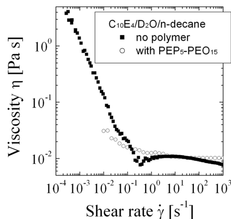
Fig. 4 The viscosity of the C_{10}E_4 microemulsion as a function of shear rate (solid symbols) compared to the same microemulsion with a PEP_5-PEO_{15} diblock copolymer (open symbols, indices give polymer molar masses in kg/mol) of Ref. [16] where erroneously the polymer influence was neglected. The steep increase at \dot{\gamma} < 0.03 \text{ s}^{-1} is a clear indication of sample surface tension, while the weak shoulder with a dip at \dot{\gamma} = 0.3 \text{ s}^{-1} indicates the presence of large structures that is also seen in the sample with polymer
