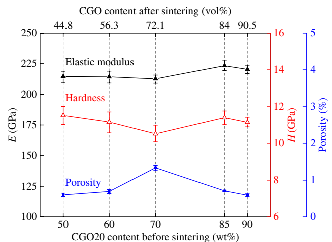
Figure 5. Elastic modulus, hardness, and porosities of CGO20–FC2O.
