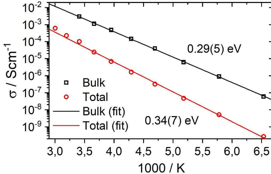
Figure 6: Arrhenius plot of the bulk and total conductivity of LATP (100 \mu\text{m} ) sintered at 920 °C.
