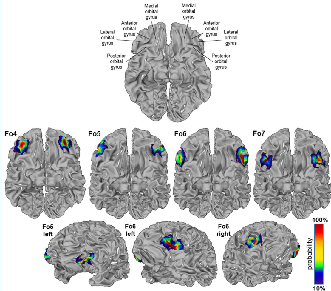
FIGURE 8 | Probability maps registered to the anatomical Montreal Neurological Institute (MNI) anatomical reference brain “Colin27”; inflated version (JuBrain atlas: https://jubrain.fz-juelich.de/apps/cytoviewer/cytoviewer.php ). Ventral views of areas Fo4–Fo7 (upper panels) and lateral views of Fo5 and Fo6 (lower panels). The probability is color-coded (red = full overlap of all 10 brains, dark blue = only one brain).
