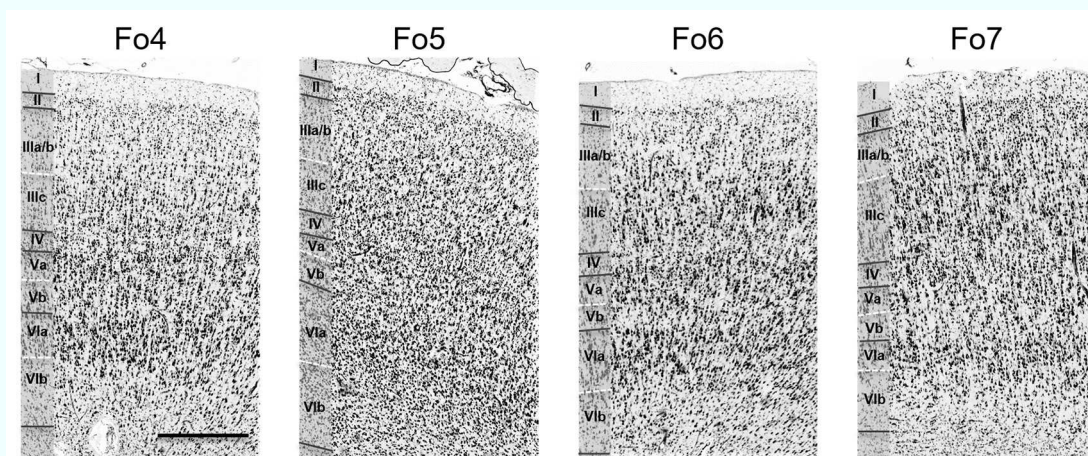
FIGURE 3 | Cytoarchitecture of areas Fo4–Fo7 in the lateral OFC. Roman numerals indicate cortical layer I to VI. Scale bar = 500 \mu m.
