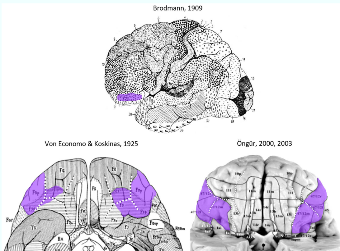
FIGURE 1 | Area 47 in the lateral orbitofrontal cortex (lateral OFC) in the human brain according to previous cytoarchitectonical analyses (Brodmann, 1909; von Economo and Koskinas, 1925; Von Economo, 1929; Öngür et al., 2003). The sulcal pattern is highlighted with white dotted lines. Images have been modified such that the sulcal patterns are highlighted with white dotted lines, and the approximate extent of Area 47 is labeled in purple.
