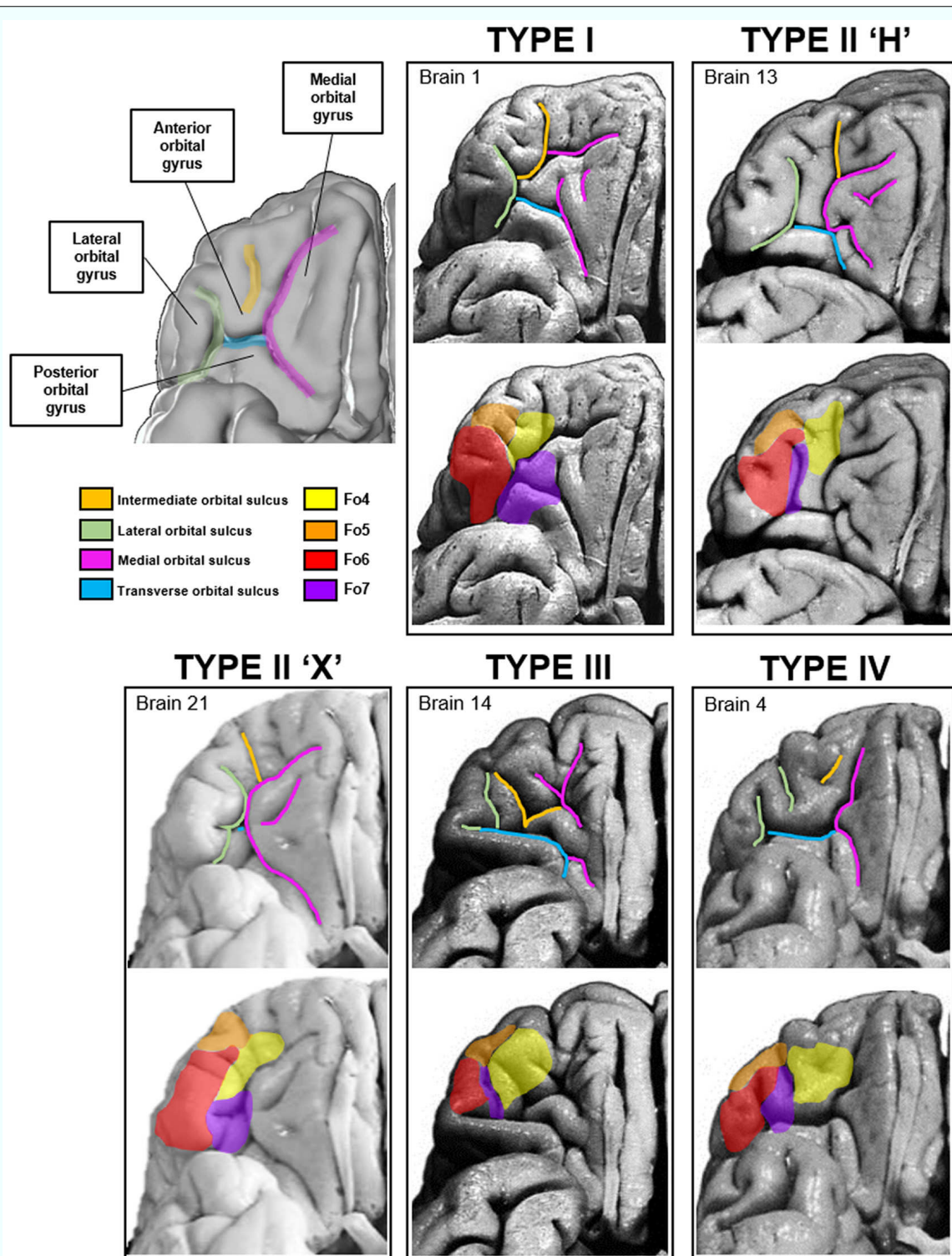
FIGURE 10 | Four types of sulci and gyri patterns in the medial and lateral orbitofrontal region of the right hemisphere have been described according to Ono, Chiavaras and Rodrigues (Ono et al., 1990; Chiavaras and Petrides, 2000; Chiavaras et al., 2001; Rodrigues et al., 2015). Localization of the respective areas differed between the four types according to the sulcal arrangements.
