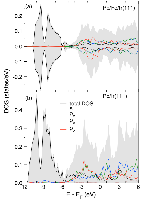
FIG. 3. (a) Orbitally resolved DOS of the Pb atoms in the honeycomb structure on Fe/Ir(111). The total Pb DOS is shown as gray background, and the s , p_x , p_y , and p_z contributions are shown in black, blue, green, and red, respectively. Positive and negative values correspond to majority and minority spins, respectively. (b) The same quantities for the Pb honeycomb lattice on Ir(111).
