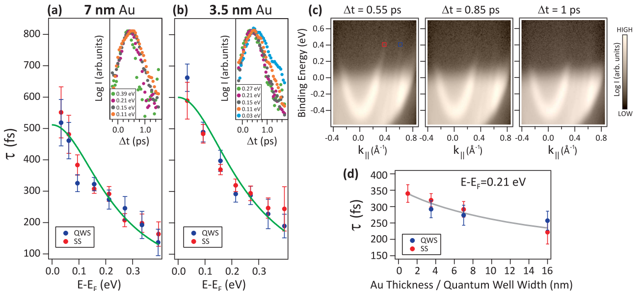
FIG. 6. (a) and (b) Decay constants of the surface state [red (light) color] and quantum-well states [blue (dark) color] for Au quantum films of (a) 7-nm and (b) 3.5-nm thicknesses. The corresponding time-resolved intensities as a function of time delay at different selected energies are shown in the insets. The data were extracted from small energy-momentum windows, such as the ones shown in (c). Green (light) solid lines are fits to the data (see the text). (c) From left to right, tr-ARPES dispersions at selected time delays ( \Delta t = 0.55, 0.85 , and 1 ps) after optical excitation. (d) Thickness dependence of the decay times at an energy of 0.21 eV above E_F . The gray solid line is a guide to the eye.
