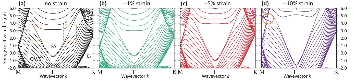
FIG. 4. Density-functional theory (DFT) calculations of the band structure of a 4 nm-thick Au slab subjected to different grades of strain. (a) No strain, (b) expansive strain of +1%, (c) compressive strain of -5%, (d) extreme compressive strain of -10%. Strain causes an energy shift of the surface state (SS) band dispersion, a change in its effective mass and a reduction of the spin splitting. The deviation from free-electron-like behavior in the SS dispersion becomes more pronounced close to the region where the SS connects to quantum-well state (QWS) bands [orange dashed rectangles in (a)]. For an extremely strained Au film in (d), the opening of an inverted band gap along the time-reversal-invariant direction \bar{\Gamma} - \bar{M} [orange circle] is shown by the connectivity of the bands.
