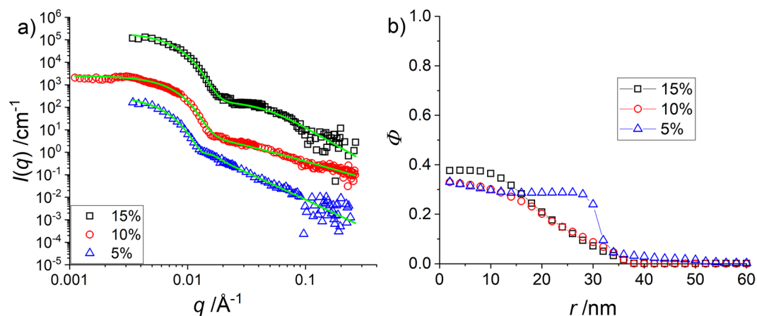
Figure 6. (a) Vertically shifted I(q) vs. q from SANS measurements of three H-pNIPMAM-core D7-pNNPAM-shell microgels with different CCC as indicated in the legend at T = 55^\circ\text{C} , under matching conditions of the shell. (b) Density profiles of core monomers determined by the multi-shell RMC approach.
