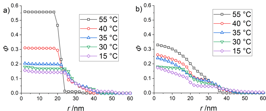
Figure 5. (a) Density profiles of the H-pNIPMAM-core with a CCC of 10 mol% in D_2O (data adapted from Cors et al. 35 (b) Density profiles of the core monomers of the H-pNIPMAM-core D7-pNIPMAM-shell system with the same core as in (a) and an index-matched shell (CCC = 1.9 mol%).
