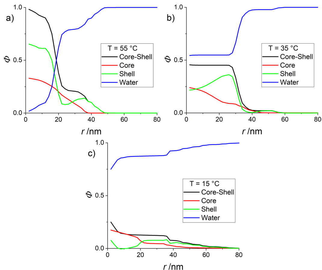
Figure 7. Density profiles of core and shell monomers, and water for H-pNIPMAM/D7-pNNPAM core-shell microgels (CCC = 10%mol) in H 2 O/D 2 O under matching conditions of the shell. (a) T = 55\text{ }^{\circ}\text{C} (b) T = 35\text{ }^{\circ}\text{C} (c) T = 15\text{ }^{\circ}\text{C} .
