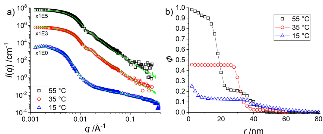
Figure 2. H-pNIPMAM core with H-pNIPMAM shell with CCC = 10 mol% at different temperatures. (a) Intensity shifted experimental data of I(q) vs. q of SANS measurements in D 2 O. The green lines indicate the multi-shell RMC fits. (b) Density profiles obtained with the RMC model.
