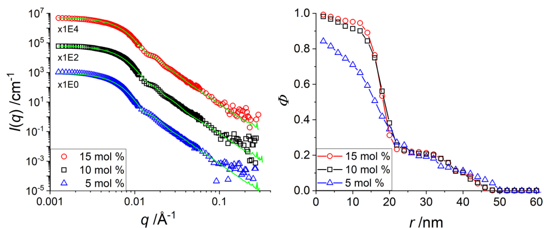
Figure 3. H-pNIPMAM core with H-pNNPAM shell with CCC = 5 mol% (blue triangles), CCC = 10 mol% (black squares) and CCC = 15 mol% (red circles) (a): Vertically shifted I(q) vs. q of a SANS measurement at 55 °C in \text{D}_2\text{O} (b): Corresponding density profiles obtained by the multi-shell RMC model.
