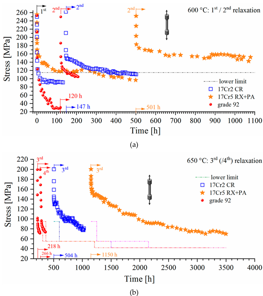
Figure 12. Stress relaxation of cold-rolled 17Cr2 and RX + PA 17Cr5 material in comparison to ferritic-martensitic grade 92, (a) 1 st + 2 nd run: 600 °C (initial stress level: 250 MPa) and (b) 3 rd + (4 th ) run: 650 °C (initial stress level: 200 MPa).
