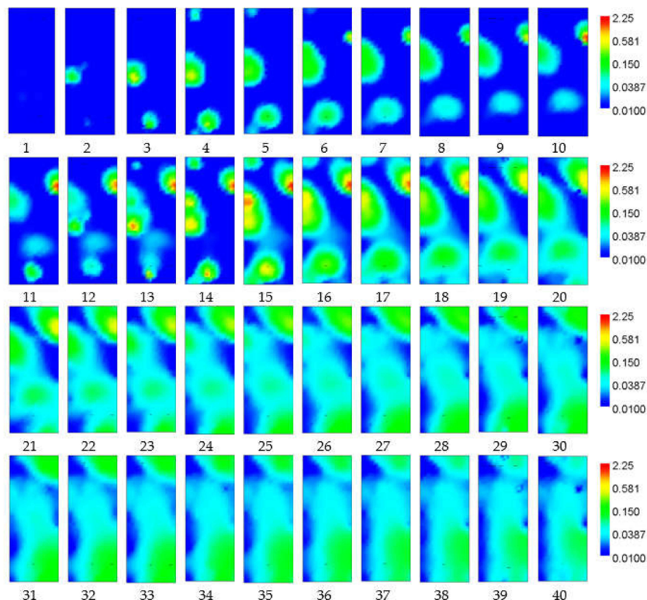
Figure 13. The spatial pattern of the atrazine concentration ( \mu\text{g/L} ) in the aquifer from year 1 to year 40 (a logarithmic color scale).
