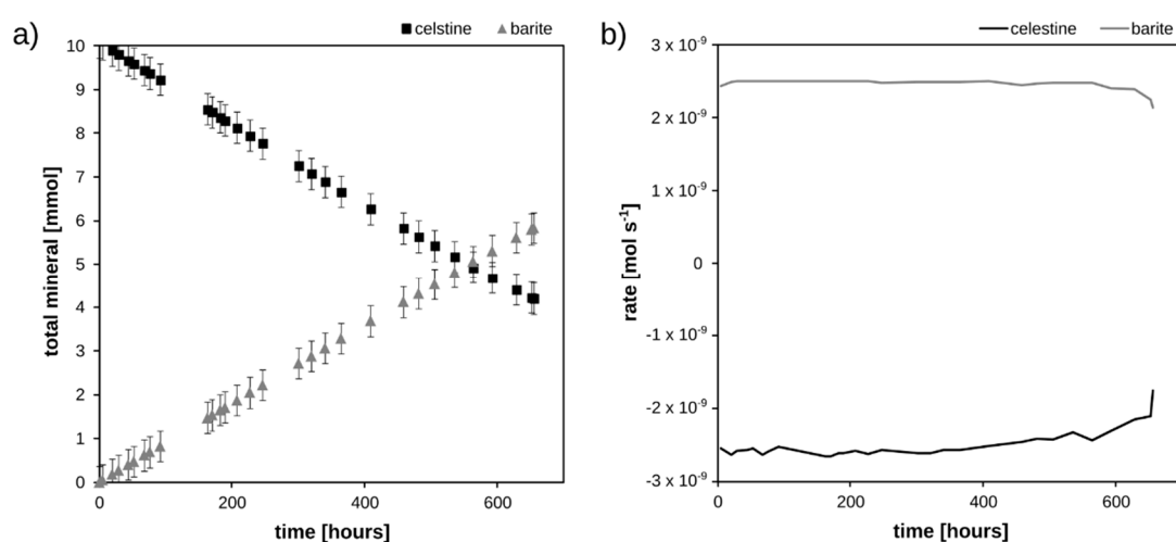
Figure 4. (a) Total amounts of minerals in the column, and (b) rates of barite precipitation and celestine dissolution as function of time.
