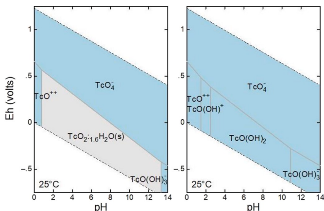
Fig. 1. Eh–pH diagram for Tc species in aqueous systems (Tc = 10^{-6} M (left), Tc = 10^{-9} M (right)). Aqueous species are shown in light blue, solids in light grey. Thermodynamic database: ThermoChimie Version 9b0; Giffaut et al., 2014; Grivé et al., 2015). (For interpretation of the references to colour in this figure legend, the reader is referred to the Web version of this article.)
