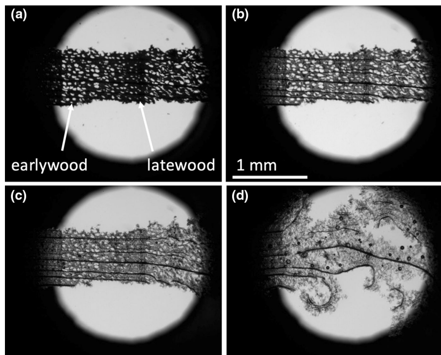
Fig. 3 Radial cut of beech (thickness 60 \mu\text{m} ) and the effect of EMIMAc at 95 ^{\circ}\text{C} at different times t = 0 s ( a ), 5 s ( b ), 50 s ( c ) and 400 s ( d ). The darker and lighter regions in the middle of
