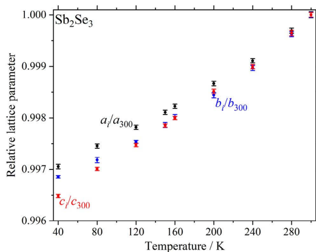
Figure 2. Temperature dependence of the normalized lattice parameter of \text{Sb}_2\text{Se}_3 . Lattice parameters at 300 K are the following: a = 11.7752(7) \text{ \AA} , b = 3.9749(2) \text{ \AA} , c = 11.6255(5) \text{ \AA} .
