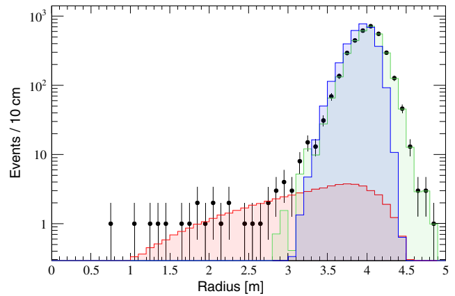
FIG. 5. Radial distribution of ^{212}\text{Bi} events occurring in the scintillator, selected with the fast ^{212}\text{Bi} – ^{212}\text{Po} coincidences, with no energy degradation for the \alpha decay (black dots). The distribution is fitted with a bulk (red) component and one from emanation and diffusion from the nylon vessel (green). The radial distribution of ^{208}\text{Tl} (blue) emanated from the vessel is derived from the latter, as described in the text.
