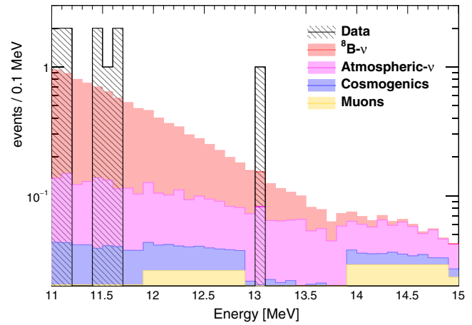
FIG. 12. FADC energy spectrum of selected events above 11 MeV, compared with the expected background spectrum.
