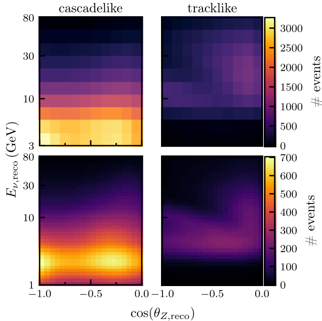
FIG. 3. Nominal expected event distributions given true NO for our analysis binning in reconstructed neutrino cosine zenith \cos(\theta_{Z,\text{reco}}) and reconstructed neutrino energy E_{\nu,\text{reco}} for the IceCube Upgrade (top) and PINGU (bottom) after 4 years of operation.
