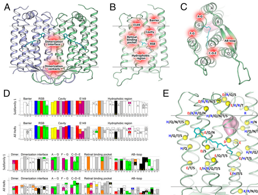
Fig. 6. Key regions of 48C12 and HeRs family identified by structure-based bioinformatic analysis. (A) View of the 48C12 dimer with identified regions (shown in red) composed of conservative residues of the dimerization interface (polar, responsible for contacts between protomers and hydrophobic, responsible for hydrophobic interaction inside the membrane). (B) View of the 48C12 protomer with the key regions (shown in red) composed of conservative residues. (C) View of the 48C12 protomer with the polar clusters (shown in red) shown to be conservative among subfamily 1 and most of other subfamilies. (D) Most conservative residues among subfamily 1 and all HeRs, comprising the key regions of 48C12. (E) The location of the residues in 48C12, which are probable analogs of charged or polar residues in other subfamilies of HeRs (selected using a sequence alignment) (SI Appendix, Figs. S16 and S17). The backbone carbon atoms of these residues are shown with yellow spheres. The polar cavity in the cytoplasmic part is shown with a pink surface. Cofactor retinal is colored teal.
