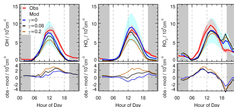
Figure 5. Mean diurnal profiles of observed and modeled OH, HO 2 , and RO 2 radical concentrations during the campaign in Wangdu in 2014. Grey areas denote nighttime and colored areas denote 1 – \sigma deviations of the mean values of observations. Model results are shown without HO 2 uptake like in the previous analysis by Tan et al. 29 and with HO 2 uptake using an effective uptake coefficient of 0.2 used by Li et al. 2019 and of 0.08 determined as an upper limit in this work. The lower panels give the differences between observations and model calculations.
