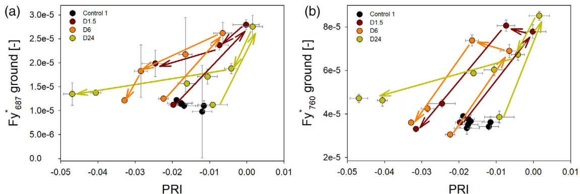
FIGURE 8 Relationship in time between PRI and the normalized sun-induced chlorophyll fluorescence measured at 687 (Fy* 687 ) and 760 nm (Fy* 760 ). The arrows indicate the time series and trends of the measurements in each plot. The error bars represent the standard deviation [Colour figure can be viewed at wileyonlinelibrary.com ]
