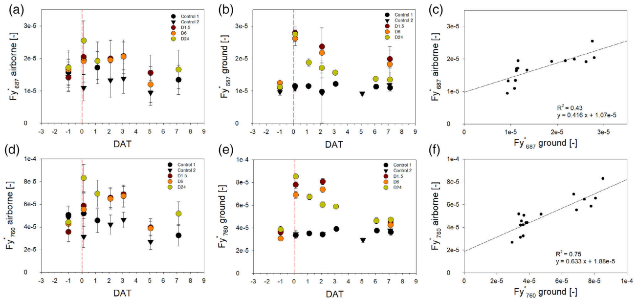
FIGURE 7 Dynamic changes of normalized sun-induced chlorophyll fluorescence (Fy*) during the experiment for all the plots estimated from airborne (a and d) and ground-based measurements (b and e). Fy* 687 (a and b) and Fy* 760 (d and e). Correlation between airborne and ground observations for Fy* 687 (c) and Fy* 760 (f). Vertical bars in airborne data represent the standard deviation of pixels within each plot. Vertical bars in ground-based data represent the standard deviation of the different point measurements taken around noon for each plot. The time of the measurements is expressed in decimal days after treatment (DAT), where DAT 0 represent the moment of the application. Data values obtained before the treatment were grouped at DAT -1 for clarity of the results [Colour figure can be viewed at wileyonlinelibrary.com ]
