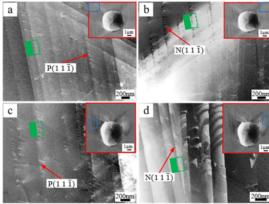
Fig. 3. ECCI images after (a) (b) indentation and (c) (d) 2 μm ploughing in the {101} grain: (a) (c) left side of imprints, i.e. domain I and (b) (d) right side of imprints, i.e. domain III: Blue frames show the corresponding precise locations of ECCI observation. (For interpretation of the references to colour in this figure legend, the reader is referred to the Web version of this article.)
