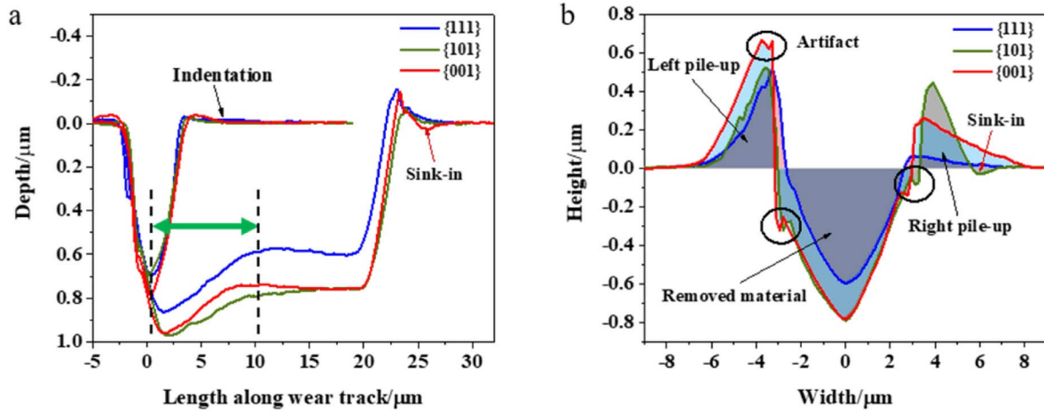
Fig. 7. Corresponding cross-sectional profiles in 20 \mu\text{m} wear tracks in the \{111\} , \{101\} and \{001\} grains: (a) shows the depth along the central line of the wear track and (b) illustrates the cross-section profile in the steady-state segment.
