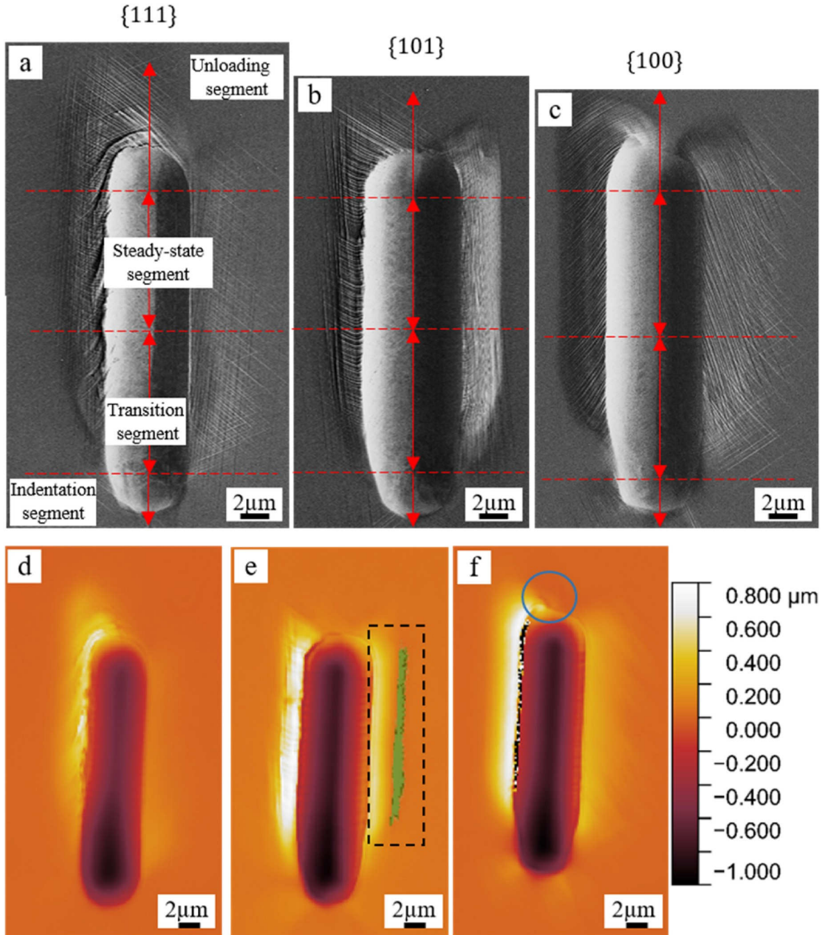
Fig. 6. (a)–(c) SEM and (d)–(f) confocal images of the wear tracks with a length of 20 \mu\text{m} . In the (a) (d) \{111\}[\bar{1}\bar{1}0] grain, (b) (e) \{101\}[011] grain and (c) (f) \{001\}[\bar{1}00] grain, which denotes the normal and wear direction.
