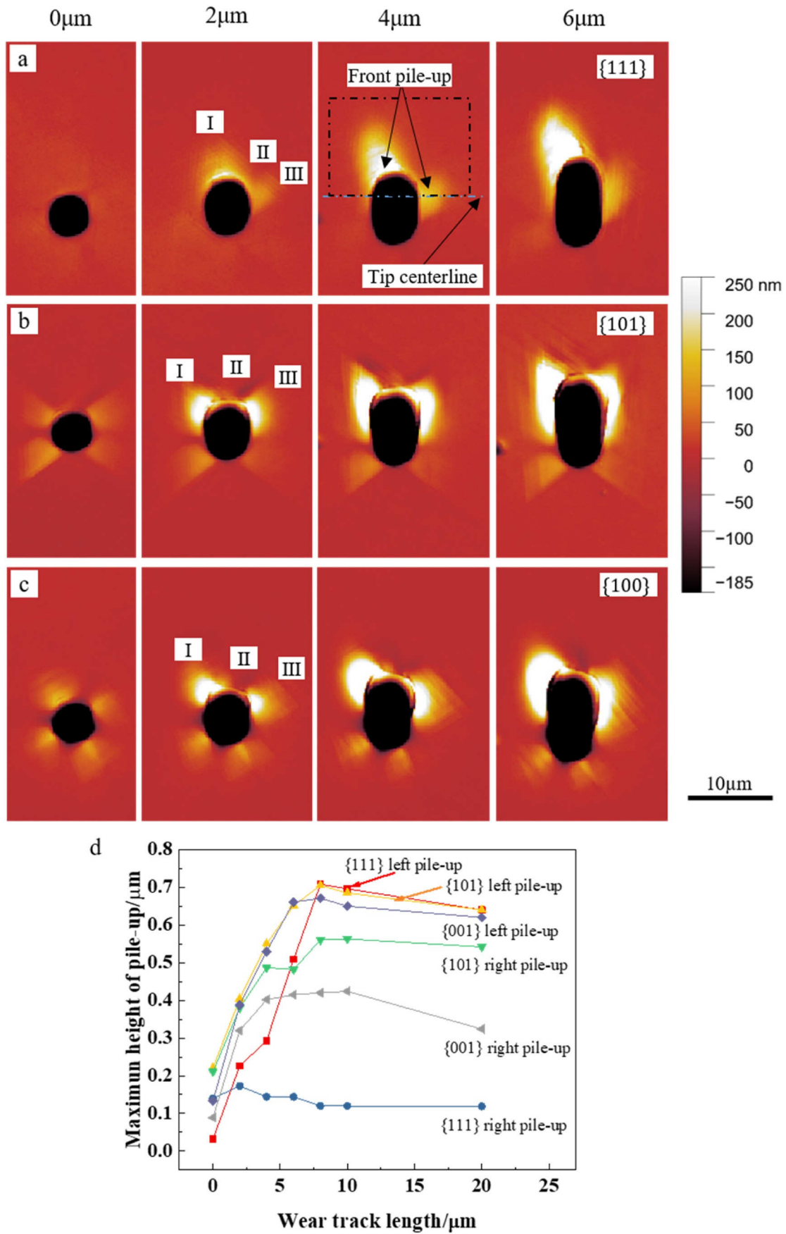
Fig. 5. Topographies after indenting and ploughing with different ploughing lengths into the (a) \{111\} grain, (b) \{101\} grain and (c) \{001\} grain. (d) shows the maximum heights of pile-ups as a function of wear track length.
