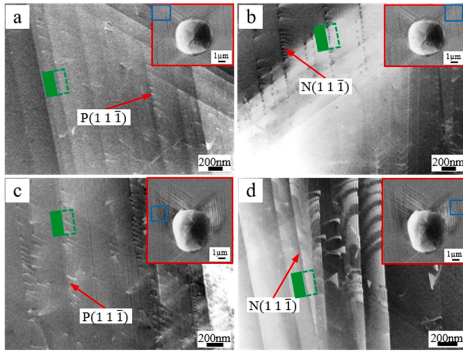
Fig. 3. ECCI images after (a) (b) indentation and (c) (d) 2 μm ploughing in the {101} grain: (a) (c) left side of imprints, i.e. domain I and (b) (d) right side of imprints, i.e. domain III: Blue frames show the corresponding precise locations of ECCI observation. (For interpretation of the references to colour in this figure legend, the reader is referred to the Web version of this article.)
