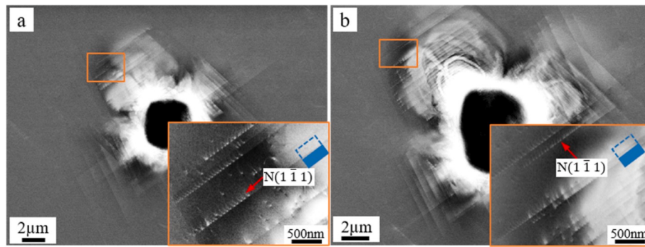
Fig. 4. ECCI images after (a) indentation and (b) 2 μm ploughing in the {001} grain.
