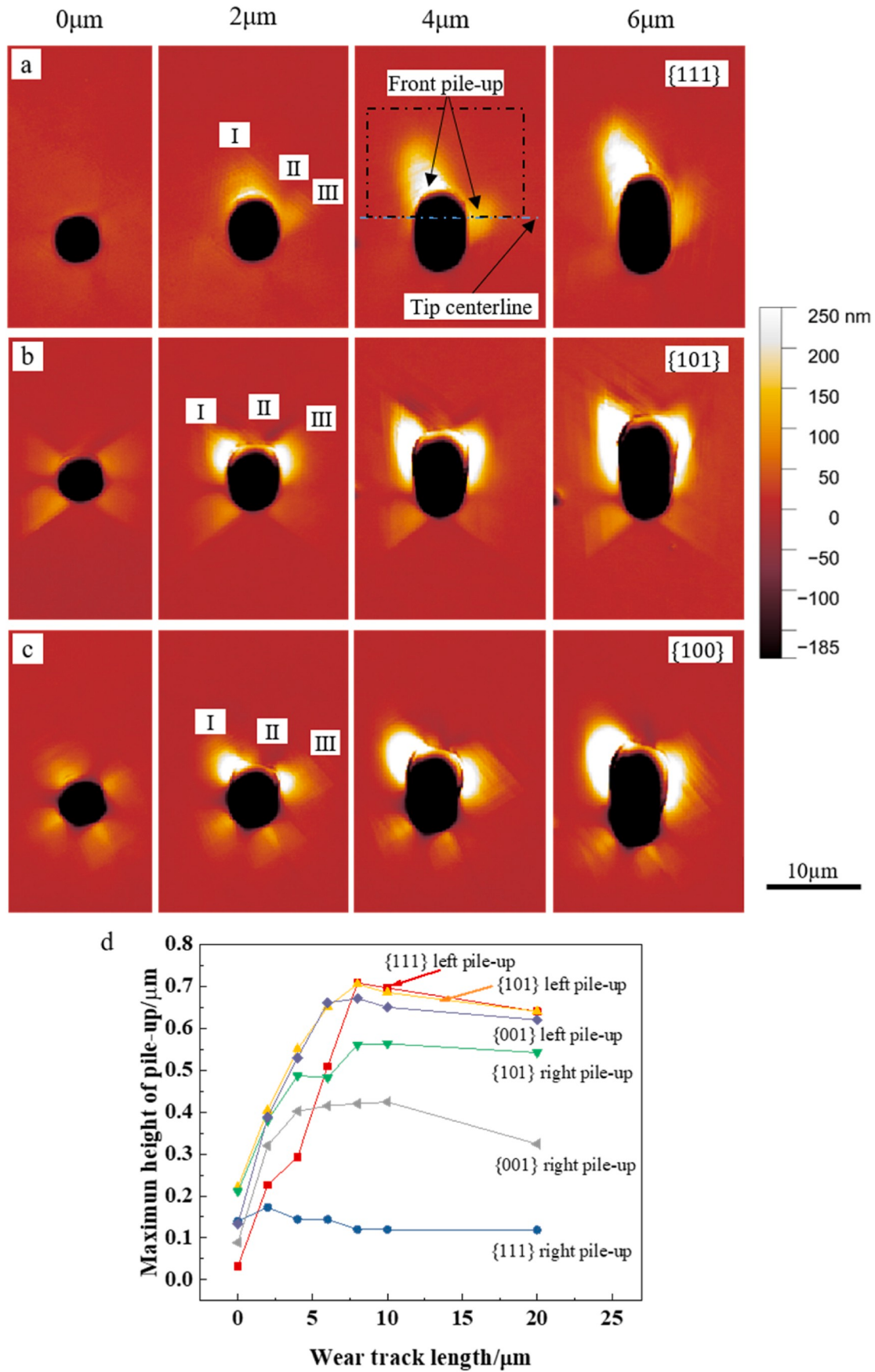
Fig. 5. Topographies after indenting and ploughing with different ploughing lengths into the (a) {111} grain, (b) {101} grain and (c) {001} grain. (d) shows the maximum heights of pile-ups as a function of wear track length.
