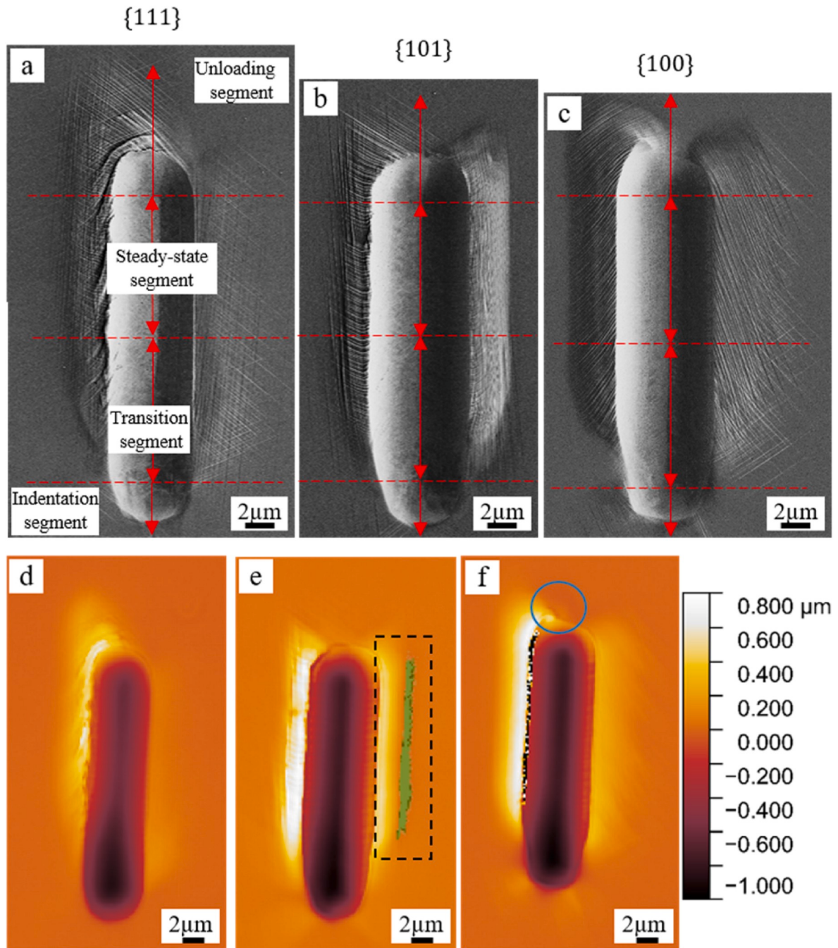
Fig. 6. (a)–(c) SEM and (d)–(f) confocal images of the wear tracks with a length of 20 \mu\text{m} . In the (a) (d) \{111\}[\bar{1}\bar{1}0] grain, (b) (e) \{101\}[011] grain and (c) (f) \{001\}[100] grain, which denotes the normal and wear direction.
