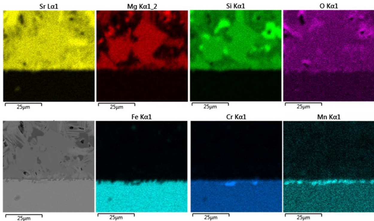
FIGURE 7 | EDX elemental mapping for the joint inferior steel-glass-ceramic 10B(Sr) treated at 800°C for 800 h.
