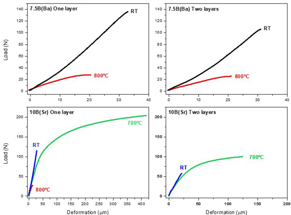
FIGURE 8 | Load-deformation curves for the bars sealing with one or two layers applied by screen printing as a function of testing temperature for compositions 7.5B(Ba) and 10B(Sr).
