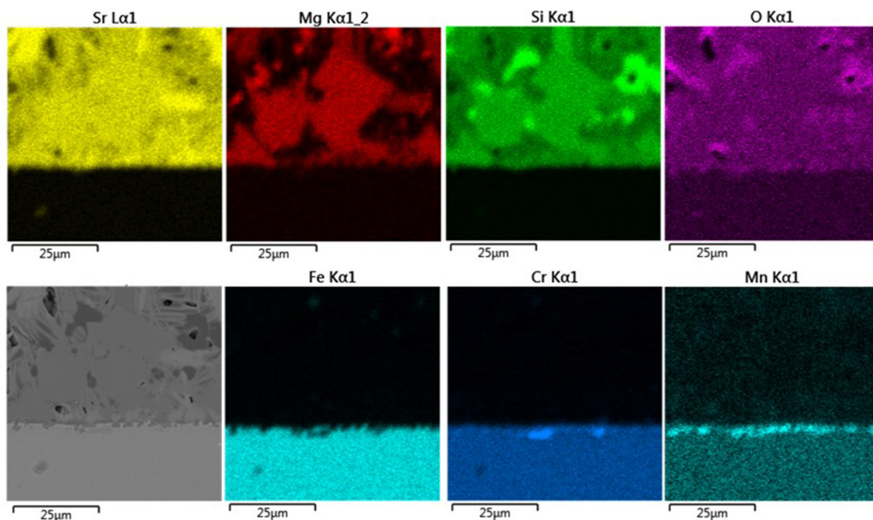
FIGURE 7 | EDX elemental mapping for the joint inferior steel-glass-ceramic 10B(Sr) treated at 800°C for 800 h.
