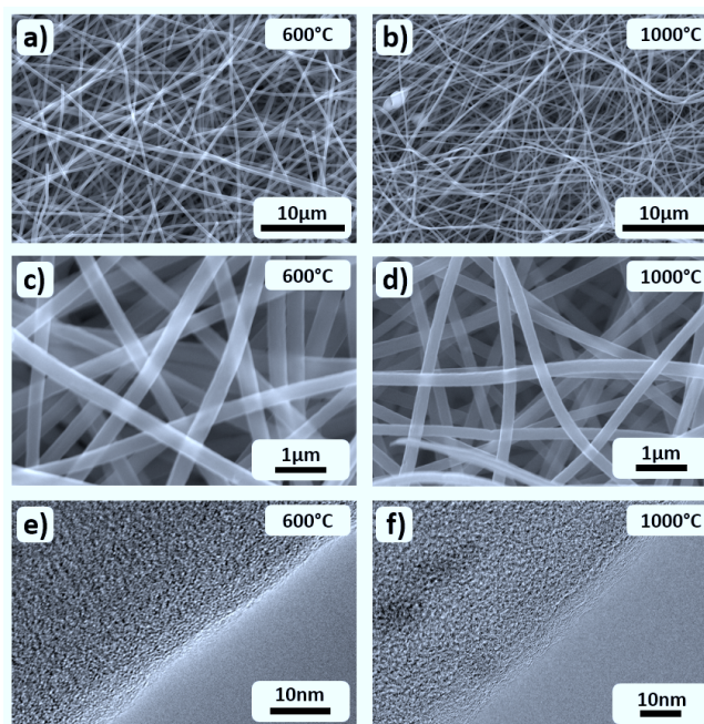
Figure 1. SEM (a–d) and TEM (e, f) images of electrospun, PAN-derived CNFs. (a), (c), and (e) Fibers that were carbonized at 600 °C. (b), (d), (f) Fibers that were carbonized at 1000 °C.
