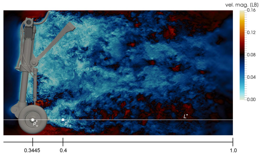
(a) Flow in the wake of the landing gear. The cross-section is located in the center between the wheels and is colored by the velocity magnitude. Furthermore, the line L^* and probe locations p_{1,2}^* at which further analyses are performed are shown.
