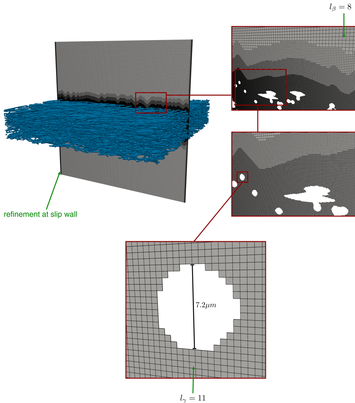
Fig. 7 Geometry and computational mesh of the GDL simulation case. The flow in a total of 27 layers is simulated. The computational mesh consists of hierarchy levels l_\alpha = 7 , l_\beta = 8 , and l_\gamma = 11 and of 2.032 \cdot 10^9 cells
