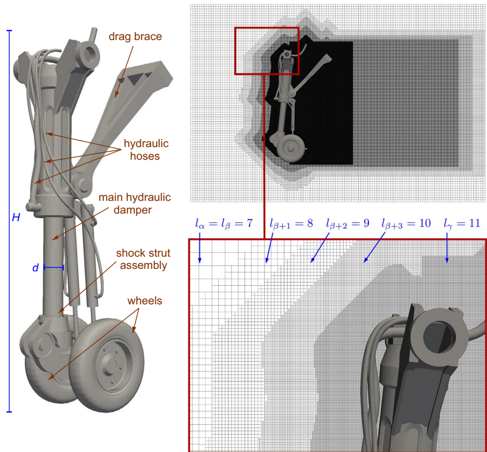
(a) Geometric setup of a front landing gear configuration of a VTOL jet airplane.
