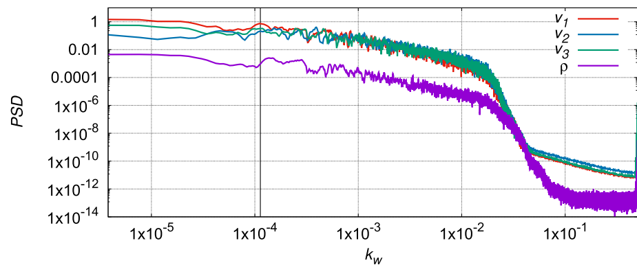
(b) Power spectral density PSD at probe location p_2^* (cf. Fig. 10a) over the wave number k_w .
