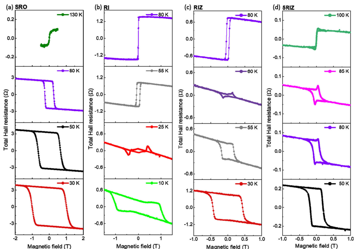
Figure 2. Hysteresis loops of the total Hall resistance at different temperatures for (a) 6 ML bare \text{SrRuO}_3 (SRO), (b) bilayer sample RI (4 ML \text{SrRuO}_3 /2 ML \text{SrIrO}_3 ), (c) trilayer sample RIZ (4 ML \text{SrRuO}_3 /2 ML \text{SrIrO}_3 /2 ML \text{SrZrO}_3 ), and (d) multilayer sample SRIZ ([5 ML \text{SrRuO}_3 /2 ML \text{SrIrO}_3 /2 ML \text{SrZrO}_3 ] _6 ), capturing the change of sign of the anomalous Hall effect around a sample-specific temperature, T_{\text{AHE}} .
