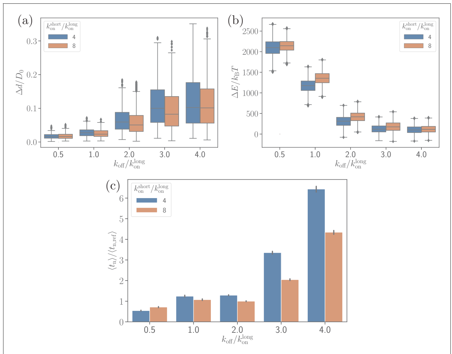
Figure 6. Effect of the off-rate k_{\text{off}} on (a) the parasite's fixed-time displacement, (b) RBC deformation energy, and (c) alignment time. Since the off-rate controls the lifetime of bonds, a smaller off-rate results in a stronger adhesion, a lower parasite displacement, and a faster alignment time. The online version of this article includes the following source data and figure supplement(s) for figure 6:
