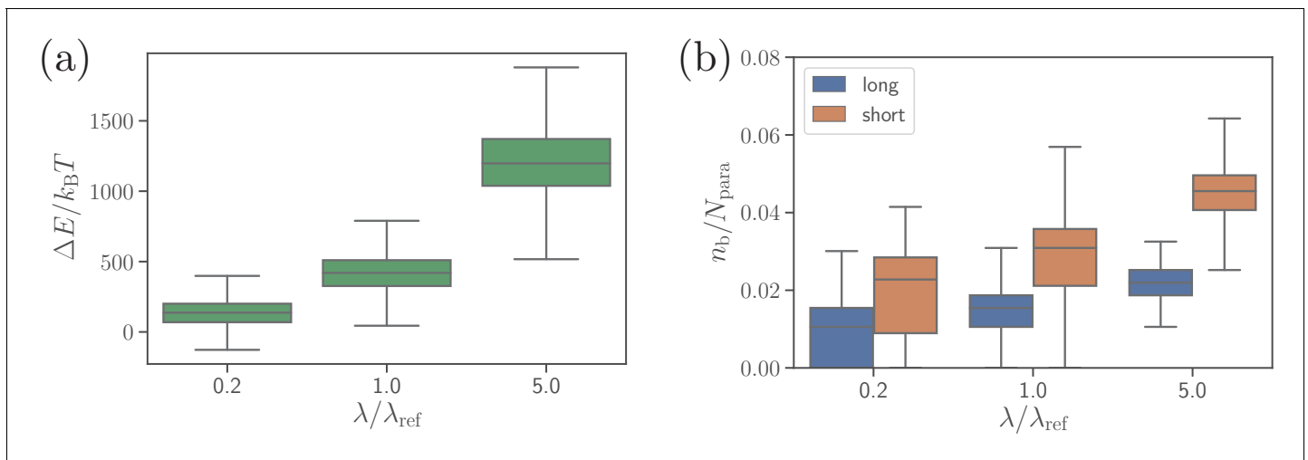
Figure 7. Effect of the extensional bond rigidities on parasite alignment. (a) RBC deformation energy and (b) the number of short and long bonds as a function of \lambda/\lambda_{ref} . \lambda_{ref} corresponds to the reference case with parameters given in Table 2 . Note that both \lambda_{long} and \lambda_{short} are changed by the same factor with respect to their \lambda_{ref} values. Here, the bond kinetic rates are k_{on}^{short} = 290.3 \tau^{-1} , k_{on}^{long} = 36.3 \tau^{-1} , and k_{off} = 72.6 \tau^{-1} . The online version of this article includes the following source data and figure supplement(s) for figure 7:
