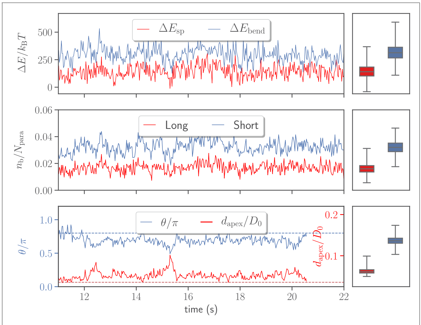
Figure 5. Variations in stretching \Delta E_{sp} and bending \Delta E_{bend} energies, the number of bonds n_b , the head distance d_{apex} , and the alignment angle \theta as a function of time for the default parameter set given in Table 2 . Temporal changes in the number of bonds are shown for both long and short bond types. The dashed lines in the bottom plot correspond to the alignment criteria in Equation 4 . For all quantities, the corresponding averages and variances represented by box plots are depicted on the right.
