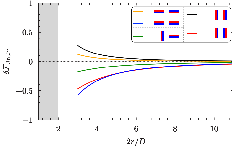
Figure 20: Large distance behavior of the interaction energy \delta\mathcal{F}_{J_n;J_n} between two Janus needles (per k_B T_c ) as function of the rescaled separation 2r/D . The shaded region corresponds to hard core repulsion of the needles in the tip-to-tip configuration.
