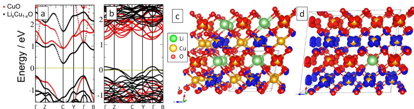
Fig. 2 Electronic band structure of lithium doped CuO for two different Li concentrations of (a) \text{Li}_{0.25}\text{Cu}_{0.75}\text{O} and (b) \text{Li}_{0.032}\text{Cu}_{0.968}\text{O} . The different numbers of bands are related to different cell sizes. The yellow line marks the Fermi level. In contrast to the insulating behaviour for x_{\text{Li}}=25\% (note the reduced band gap w.r.t. bulk CuO), the valence bands crossing the Fermi level for x_{\text{Li}}=3.2\% indicate p-type conductivity. Spin density of lithium doped CuO in two different Li concentrations of (c) \text{Li}_{0.25}\text{Cu}_{0.75}\text{O} and (d) \text{Li}_{0.032}\text{Cu}_{0.968}\text{O} (Isosurface of 0.01 \text{ e}/\text{\AA}^3 ). Majority and minority spin densities are shown by blue and red, respectively. Note the significant contribution of oxygen for the low Li doping concentration of 3.2\% .
