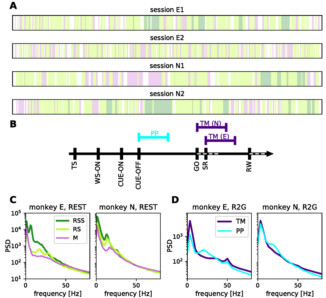
Figure 1. Behavioral segmentation in REST and R2G recordings. (A) Order and relative duration of the behavioral states defined within each REST session (single second precision): resting state (RS, light green) represents no movements and eyes open, sleepy rest (RSS, dark green) represents no movements and eyes (half-)closed, spontaneous movements (M, pink) represent movements of the whole body and limbs. (B) Order and timing of events within a single trial of an R2G session. Colored lines above the time axis indicate time intervals considered for the analysis: preparatory period (PP, cyan) and task-induced movements (TM, purple). SR indicates the switch-release event—beginning of the hand movement. PP was defined as [CUE-OFF, CUE-OFF+500 ms], and TM as [SR, SR+500 ms] for monkey E, and [SR-150 ms, SR+350 ms] for monkey N (different for the two monkeys due to differences in performance speed). (C and D) Power spectral density of LFP in different behavioral states. Panels in C pertain to REST, panels in D to R2G, left for monkey E and right for monkey N, respectively. States are defined in A and B. The peak at 50 Hz in the R2G spectra is an artifact (line frequency) and was not considered.
