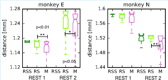
Appendix 2 Figure 1. Spatial arrangement of active SUs on the Utah array. Box plots of the radial spatial distance to the center of mass for the two REST recording sessions of monkey E (left panel) and N (right panel).
