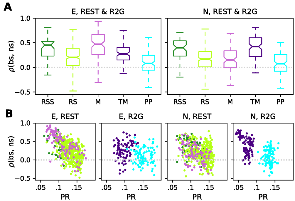
Figure 6. Instantaneous balance and its relation to dimensionality. (A) Box plots of the correlation between putative excitatory and inhibitory population activity calculated in 3 s slices, which quantifies the instantaneous (100 ms) balance for monkey E (left) and N (right). (B) Scatter plots showing the relationship between the instantaneous balance \rho(\text{bs, ns}) and dimensionality PR, for monkey E (panels on the left) and N (panels on the right). Each dot represents the PR and \rho(\text{bs, ns}) values of one 3 s slice during REST or R2G recording. Results are pooled across all recordings of the respective type.
