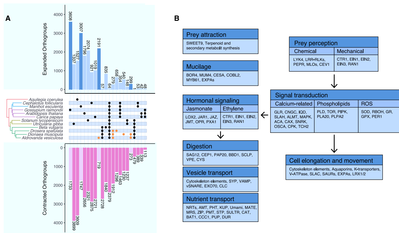
Figure 2. Gene Family Expansion and Contraction
