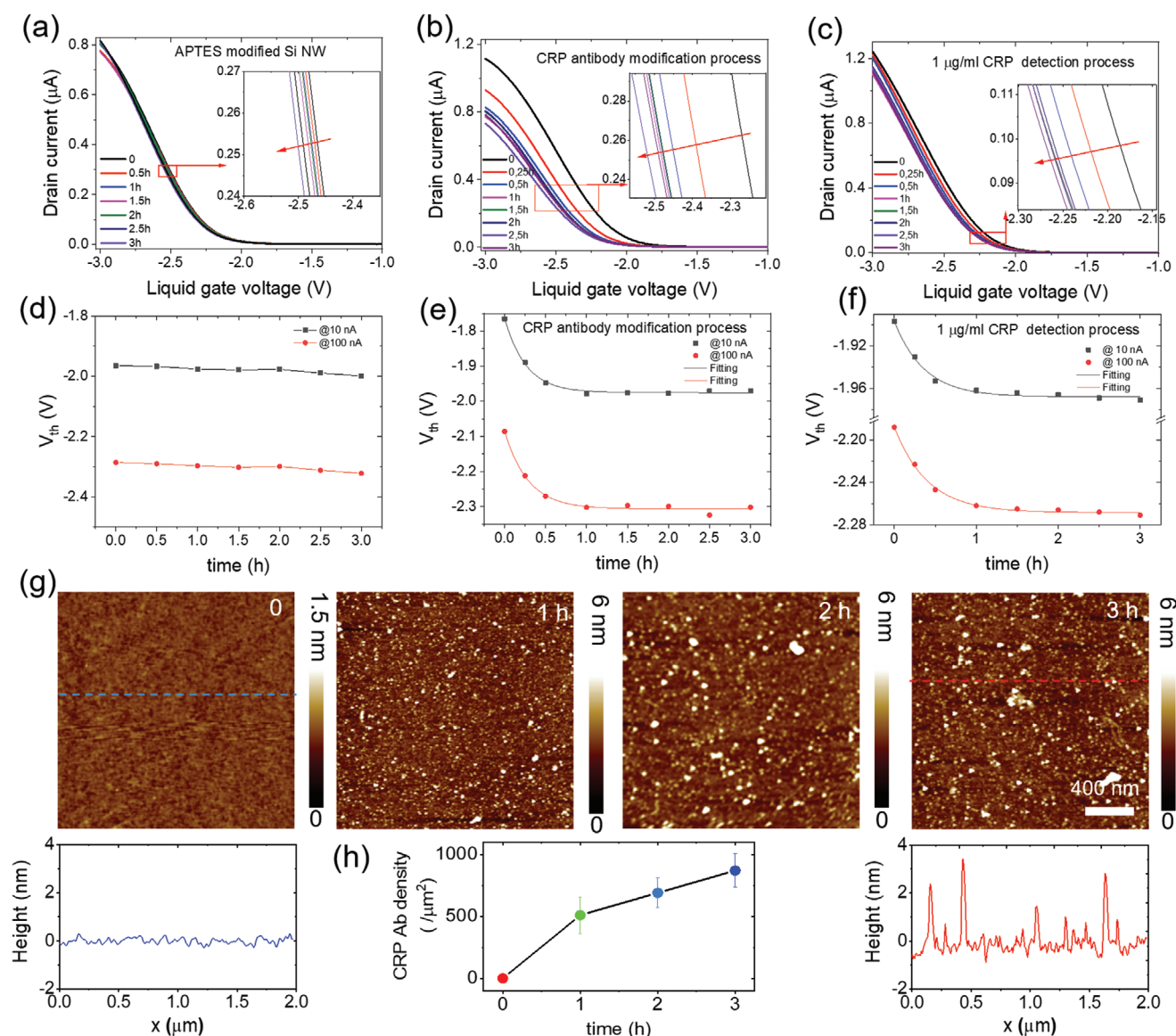
Figure 2. Long-term measurements of I - V characteristic shift of Si NW FETs in 1 \times 10^{-2} M PBS solutions with pH = 7.4 during different stages: a) after APTES modification; b) during 1 \mu g mL ^{-1} CRP antibody modification process; c) during 1 \mu g mL ^{-1} CRP antigen detection process; inner figures are zoomed in part; (d)–(f) are extracted gate voltage at constant current 10 nA (black squares) and 100 nA (red dots), and solid curves in (e) and (f) are exponential fittings for each data set from (b) and (c), respectively; g) AFM characterization of 1 \mu g mL ^{-1} CRP antibody modification process with different times, from 0 to 3 h with an interval of 1 h, and insets under 0 and 3 h are sections of cut lines showing the roughness of the APTES-modified substrate surface and CRP-antibody-modified surface, respectively; h) plot of CRP antibody surface density as a function of modification time from (g) with error bars.
