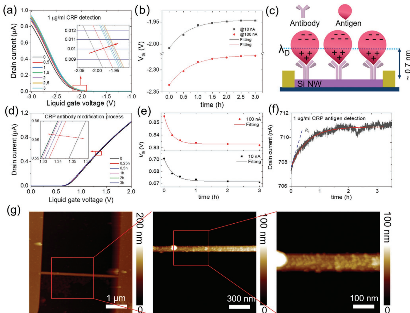
Figure 4. a) I - V characteristics of p-type Si NW FETs measured during 1 \mu\text{g mL}^{-1} CRP antigen detection process in 1 \times 10^{-2} M PBS pH 8.4; inset in (a) shows zoomed part of V_{\text{th}} shift with time; b) extracted gate voltage at a constant current of 10 nA (black squares) and of 100 nA (red dots) from (a); c) schematic of closest binding site charge dominating the gating effect on the NW surface; d) I - V characteristics of n-type Si NW FETs measured in 10 \times 10^{-3} M PBS solutions with pH = 7.4 during CRP antibody bonding process; inset to (d) shows zoomed part of shift of I - V characteristics to low voltage range with time; e) extracted gate voltage at a constant current of 10 nA (black squares) and of 100 nA (red dots) from (d), and red solid line is exponential fitting; f) time trace of 1 \mu\text{g mL}^{-1} CRP antigen detection process, V_{\text{ds}} = 0.1 V, V_{\text{lg}} = 1.5 V, red solid line is exponential fitting of time trace, and blue dashed line shows the binding rate ( k_1 ) of 1 \mu\text{g mL}^{-1} CRP antigen to antibody at the very beginning of the binding process; g) AFM characterization of CRP biomarkers on NW (200 nm width and 4 \mu\text{m} length) after long-time detection with zoomed part to show the CRP protein complex on silicon nanowire surface.
