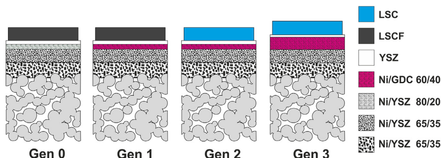
Figure 6. Stepwise Optimization of Processing and Microstructure of the Metal-Supported Solid Oxide Fuel Cell (Plansee SE concept)
