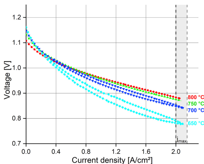
Figure 3. Electrochemical Performance of Gen 3 Cells
