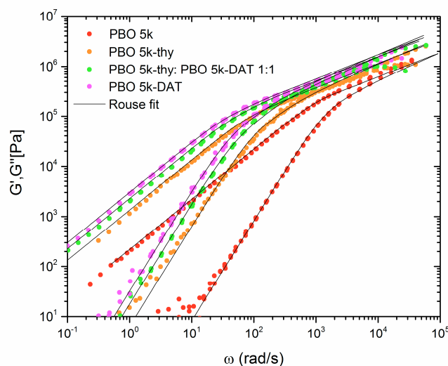
Figure 4. Storage G'(\omega) and loss modulus G''(\omega) master curves, reduced to T_0 = -25^\circ\text{C} of unfunctionalized and functionalized PBO-5k compounds. Fits to the Rouse model are included.
