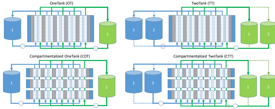
Fig. 1: Scheme of the different design configurations for a VRFB under investigation in this study considering additional tanks or compartmentalization. The OT configuration represents the state of the art.
