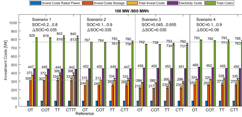
Fig. 10: Results of investment costs calculation for j = 200\text{mA}/\text{cm}^2 of each configuration at 100MW - 800MWh in each Scenario. Uncertainty in investment costs for tanks result in uncertainty of investment costs for rated power, total investment costs and total costs and are indicated by the black bar-lines (The numbers are given for maximal values).
