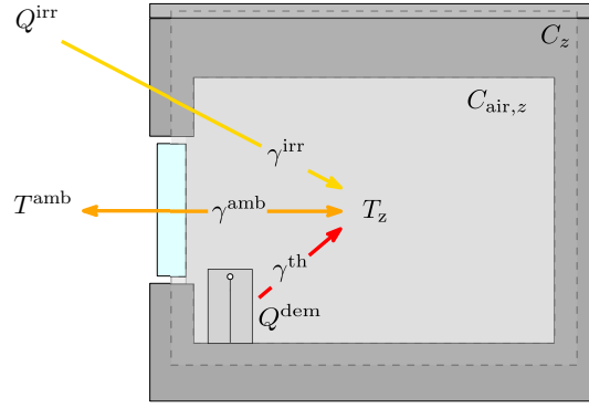
Figure 9: Heat flow scheme for building with relevant contributions
