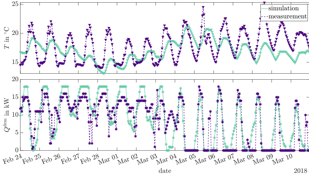
Figure 3: Comparison of simulation and measurements for the original experimental facility “EF 1”
