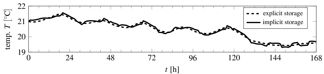
Figure 8: Internal temperature of Building "OB1" based on simulated heat input and simulated heat input plus optimized heat transfer rate of TES
