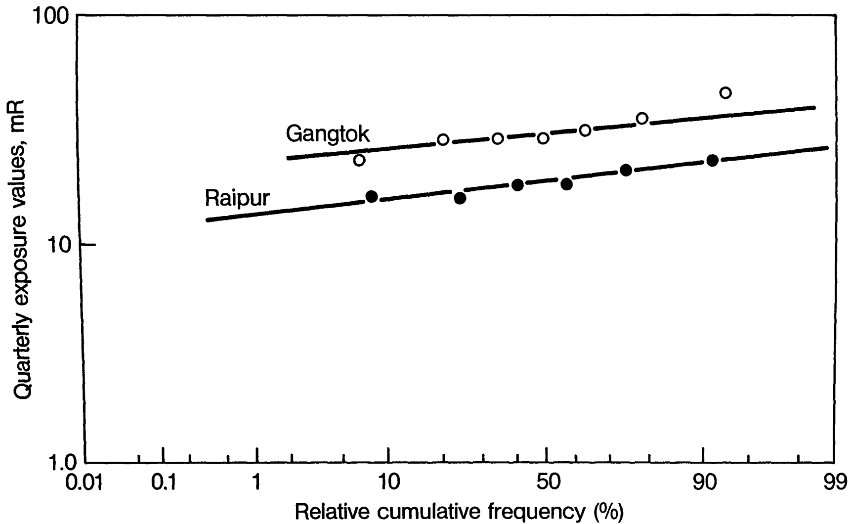
Figure 1: Log probability plots of quarterly background radiation levels at Raipur and Gangtok (Period of monitoring: 6 & 7 consecutive quarters respectively)
