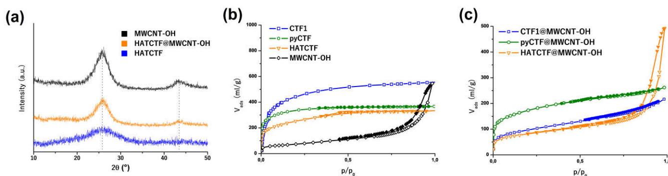
Figure 3: (a) PXRD patterns of MWCNT-OH, HATCTF and HATCTF@MWCNT-OH (b) N 2 -physorption of the MWCNT, CTF1, pyCTF, HATCTF (c) N 2 -physorption of the respective hybrid materials
