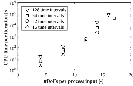
Figure 7: CPU time per iteration of the adaptive grid algorithm vs. DoFs for optimization for each of the process inputs. Note that there are four process inputs m_t^E , m_t^C , y_t^E , and y_t^C with equal mapping matrices. Symbols depict the varying scheduling horizons (upwards-pointing triangles: 16 h, circles: 32 h, squares: 64 h, downwards-pointing triangles: 128 h).
