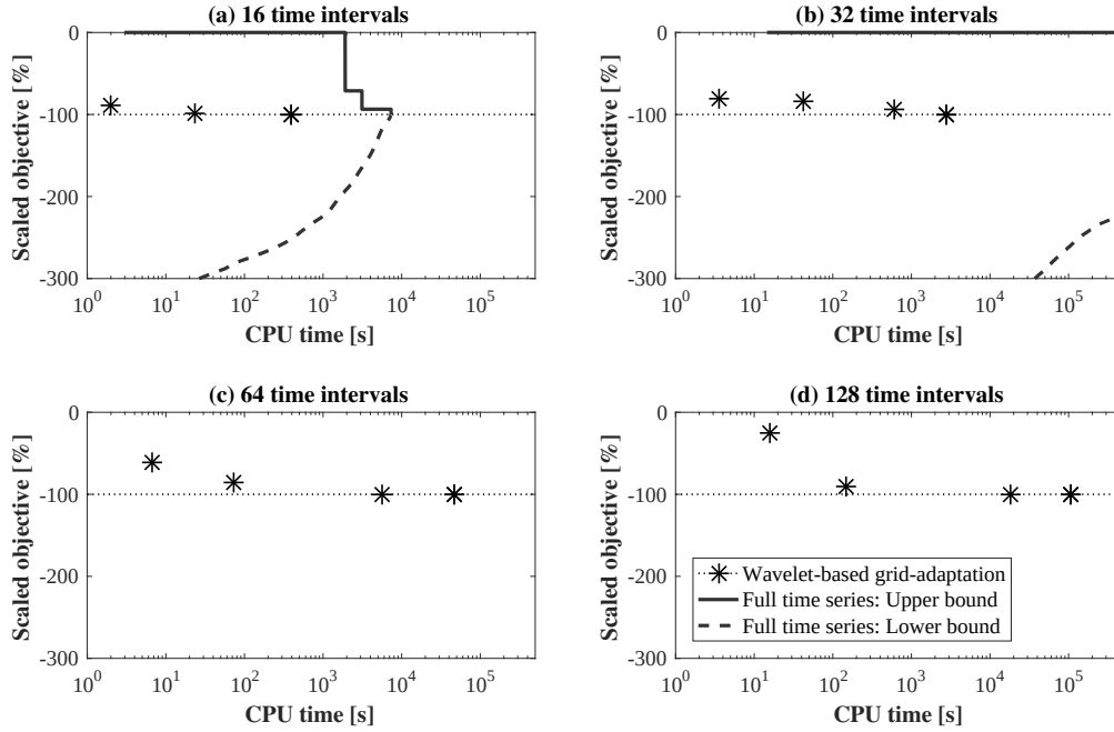
Figure 4: Progress of the grid-adaptation and comparison to a global optimization considering individual DoFs for each interval of the time series. Results are depicted for T = 16, 32, 64, 128 ((a) - (d)). Objective function values are relative to the best feasible point furnished by the algorithm (dotted line). Asterisks depict the outcome of the algorithm after each iteration. The solid lines give current upper bounds and dashed lines current lower bounds when solving the problem considering individual DoFs for each interval.
