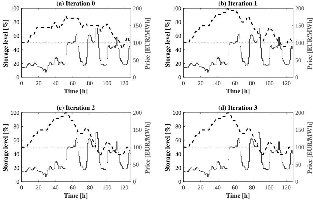
Figure 5: Operation schedule of the CAES plant after each of the four iterations of the grid-adaptation ((a) - (d)) for a scheduling horizon of T = 128 . Dashed thick black lines depict the storage level (i.e., the cavern pressure), solid thin gray lines correspond to the electricity price profile for the case study. The dotted line depicts the production target.
