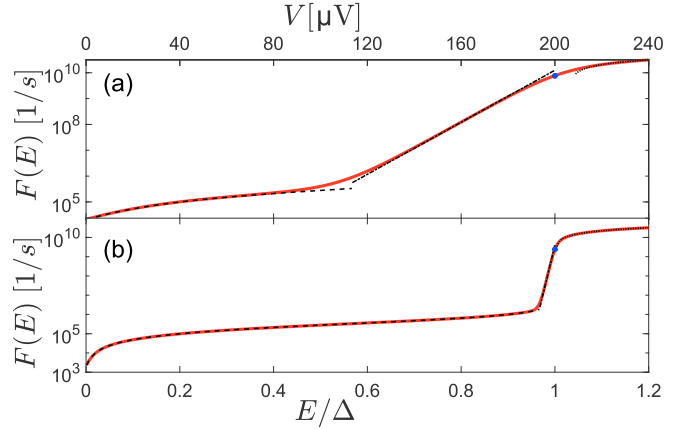
FIG. 11. Normalized tunneling rate F(E) as a function of the bias energy E at the electron temperature (a) k_B T_N / \Delta = 0.043 and (b) k_B T_N / \Delta = 0.0043 . Black dashed lines represent the approximate results from Eq. (A2) for E < E_{co} . Black dash-dotted lines are from Eq. (A3) for E_{co} < E < \Delta . Black dotted lines are from Eq. (A1) for E > \Delta + k_B T_N . Blue dots are Eq. (A5) for E = \Delta . The Dynes parameter is \gamma_D = 10^{-5} .
