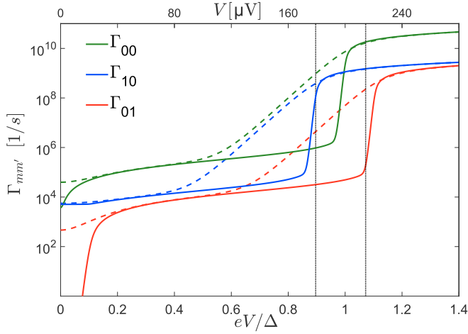
FIG. 5. Transition rates \Gamma_{mm'} as a function of the bias voltage V in a combined QCR and transmon system for the normal-metal electron temperature T_N = 100 mK (dashed lines) and T_N = 10 mK (solid lines). The vertical black dotted lines denote, from left to right, the on voltage in the thermal activation regime eV = \Delta - \hbar\omega_{10} and the on voltage in the low-temperature regime eV = eV_{\max} of Eq. (19) at T_N = 10 mK. The transmon and QCR parameters are given in Table I.
