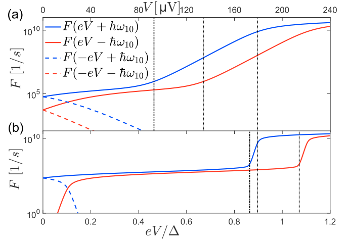
FIG. 12. Shifted normalized tunneling rate functions F(eV \pm \hbar\omega_{10}) as functions of the bias voltage V at the electron temperature (a) k_B T_N / \Delta = 0.043 and (b) k_B T_N / \Delta = 0.0043 . The vertical dash-dotted lines at eV = E_{co} - \hbar\omega_{10} bound the off-state regime from above. The region between the vertical dotted lines corresponds to low effective temperature. In panel (a), where T_N > T_N^{\text{co}} , the vertical dotted lines are at voltages eV = E_{co} + \hbar\omega_{10} and eV = \Delta - \hbar\omega_{10} . In panel (b), where T_N < T_N^{\text{co}} , the vertical dotted lines are at eV = \Delta - \hbar\omega_{10} and eV = E_{co} + \hbar\omega_{10} . The Dynes parameter is \gamma_D = 10^{-5} and the shift frequency is \hbar\omega_{10} / \Delta = 0.1 .
