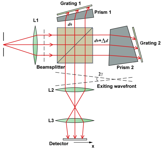
Fig. 1. Schematic of a field-widening DASH interferometer. L1 denotes the fore optics, L2 and L3 denote the exiting optics, and the arrow denotes the x direction on the detector. d_0 and d_0 + \Delta d represent the optical paths from the beamsplitter to the gratings on the arm one and arm two, respectively.
