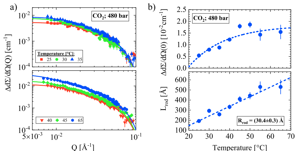
Figure 4. (a) Scattering patterns show rod-like droplets for all temperatures. (b) A linearly increasing length and constant cross-section of radius of (30.4 \pm 0.3) Å is found with increasing temperature. This experiment was extended to 20 m sample-to-detector distance thereby allowed the determination of larger L_{\text{rod}} .
