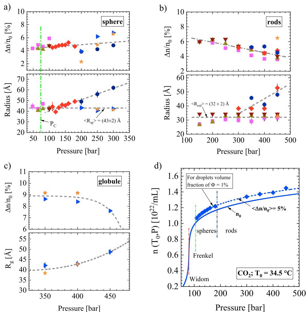
Figure 3. Relevant parameters of droplets. The parameter \Delta n/n_0 represents the relative change of CO 2 number density of the droplets with respect to the fluid number density n_0 assuming a droplet volume fraction of \Phi = 1\% . \Delta n/n_0 is plotted as a function of pressure. The symbols correspond to the following temperatures: 12 °C (■), 20.5 °C (▲), 27.2 °C (▼), 34.5 °C (◆), 52 °C (●), 56 °C (◐), 66 °C (★). (a) In the lower part of the figure, the radius of all the observed spherical droplets analyzed with the form factor of spheres in Eq. (7). Whereas \Delta n/n_0 increases slightly with an overall average value of (1.67 \pm 0.06)\% , the radius splits into two parts above 130 bar. The radii below 56 °C increase linearly later transforming into rod-like droplets, whereas the radii at 56 °C and 66 °C remain constant forming a globular morphology at higher pressure. (b) \Delta n/n_0 and radius of the rod cross-section. \Delta n/n_0 shows a slightly linear decline with pressure, which might indicate reduced droplet volume fraction. An appreciably larger cross-section of the rods ( R_{rod} ) is determined at higher pressure for 34.5 °C and 52 °C. (c) \Delta n/n_0 and the radius of gyration ( R_g ) of the globular droplets declines and increases slightly, respectively. (d) Number density at T = 34.5 °C versus pressure (taken from Ref. 18 ). For droplets assuming \Phi = 1\% volume fraction, an averaged 5% enhanced number density is obtained. In the case of \Phi = 10\% , a \sqrt{0.1} smaller value of \Delta n/n_0 of \sim 1.6\% is obtained.
