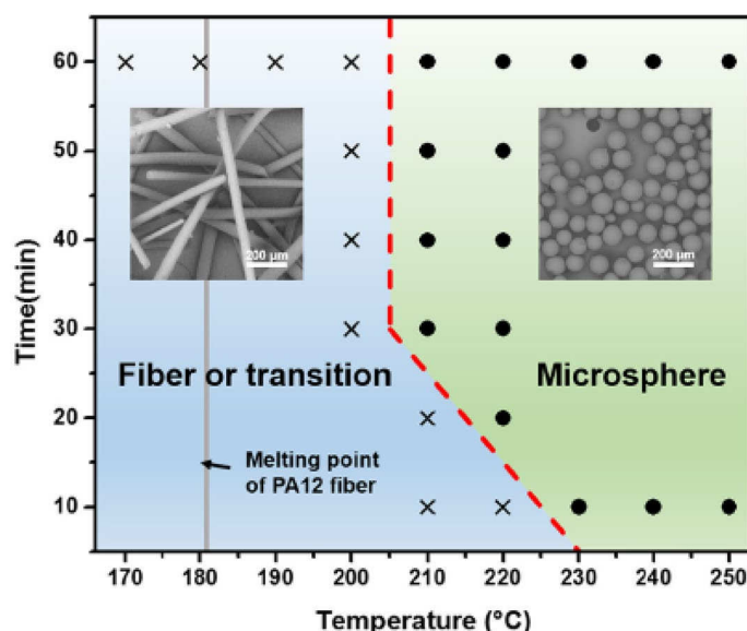
Figure 5. Temperature–time morphology diagram illustrating the sample morphology of PA12 (Polyamide) fibers ( D_0 = (32.6 \pm 3.6 \mu\text{m}) ) after thermal treatment in the PEO (Poly(ethylene oxide) matrix. The cross represent fiber or beads-on-string morphologies and the circles represent microsphere morphologies. The grey line shows the melting point of PA12 fiber. [Figure and text from Ref. 33 (Fig. 6)].
