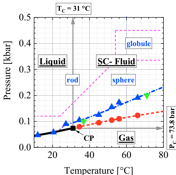
Figure 1. Temperature–pressure plane of the CO 2 phase diagram. The solid line represents the gas–liquid phase boundary with the critical point (CP) at its endpoint T_C = 31\text{ °C} and P_C = 73.8\text{ bar} . The solid grey lines with an arrow represent the borderlines of gas, liquid, and supercritical (SC) fluid phases. The dashed and dashed-dotted lines, respectively, show the Widom (●) and Frenkel (▲ (isotherm), ▼ (isobar)) lines, and the symbols show the corresponding SANS values. The Widom and Frenkel lines represent the locations of the largest degree of thermal molecular density fluctuations and the onset of droplet formation, respectively. Droplets of different shapes form beyond the gas–liquid and Frenkel line representing a liquid–liquid phase transition of phases with the same composition but different molecular densities. Such phase transition obeys the class of polymorphic phase transition of one-component disordered systems such as liquids and glasses, whose most prominent representative is water.
