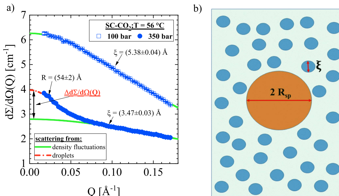
Figure 2. SC-CO 2 at 56 °C: scattering cross-section and schematic image. (a) Scattering pattern below the Widom line ( P_W = 110 bar) at 100 bar showing only scattering from thermal density fluctuations according to the Ornstein–Zernicke law in Eq. (2) (solid line). On the other hand, scattering at 350 bar shows scattering (dashed-dotted line) from thermal density fluctuations (solid line) and in addition from droplets (double arrow) analyzed with Eqs. (6)–(9). Both contributions superimpose incoherently, i.e. their intensities are added. The Frenkel line was determined at (173 \pm 10) bar. (b) The schematic image shows thermal fluctuations of correlation length \xi and a droplet of radius R_{sp} in accordance with d\Sigma/d\Omega(Q) at 350 bar in (a) .
