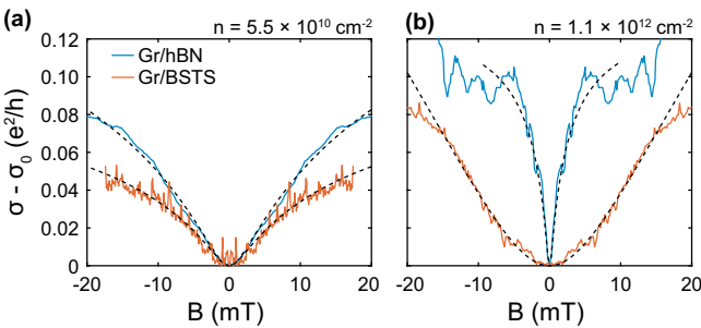
FIG. 3. WL measurements Gr/hNB (blue) and Gr/BSTS (red) (a) close to CNP and (b) at high densities ( n = 1.1 \times 10^{12} \text{ cm}^{-2} ). The dashed lines are fits to the McCann model for WL in Gr for both panels.
