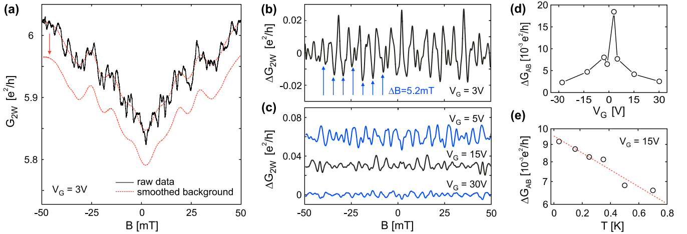
FIG. 2. (a) Solid black line: G_{2W} as a function of B at V_G = 3 V. Red dashed lines show \langle G_{2W} \rangle used for background subtraction. For clarity the trace is duplicated with an offset (see red arrow). (b) and (c) Processed data with \Delta G_{2W} for various V_G . Vertical arrows in panel (b) indicate a periodicity of \Delta B_{AB} = 5.2 mT. In panel (c) the traces are plotted with an offset for clarity. (d) \Delta G_{AB} as a function of V_G . All these measurements are taken at T = 36 mK. (e) \Delta G_{AB} as a function of T at V_G = 15 V. Red dashed line represents an exponential fit to the data \Delta G_{AB} \propto \exp(-T/T_0) with T_0 = 1.75 K.
