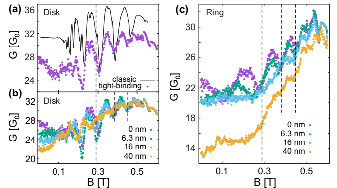
FIG. 8. (a) A comparison of the tight-binding result for the transmission to a simple classical description at a Fermi energy E_F = 98 meV for the transport through a disk ( r_i = 0 ). A correspondence of the features in the two calculations is visible all the way up to the quantum Hall limit w = 2r_C . Note that the results also approximately match the results of Fig. 7(b) for w \gtrsim r_C indicating that the inner radius has only an effect for small cyclotron radii. (b) Simulation of the disk geometry with a sinusoidal modulation of the outer radius with amplitude \delta r = 0, 6.3, 16 , and 40 nm. The conductance for the disk is shown for different strength of edge roughness with the result that the position of the conductance minima are rather robust to edge roughness. (c) Finally, we also include edge roughness in the simulation of the graphene ring. We observe that with increasing edge roughness the features of quantization and magnetic focusing weaken until they resemble a shoulder-like structure that was observed in the experiments.
