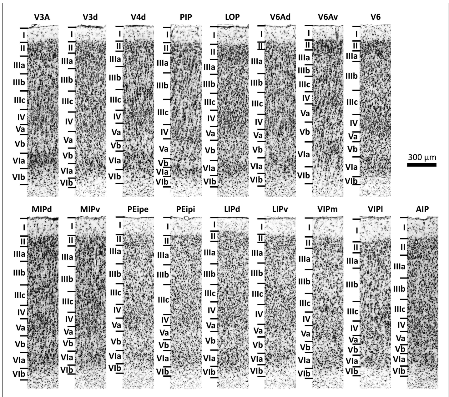
Figure 4. Cytoarchitecture of the 17 IPS areas. Scale bar 300 \mu m. Roman numerals indicate cytoarchitectonic layers. For abbreviations, see Figure 2 .
