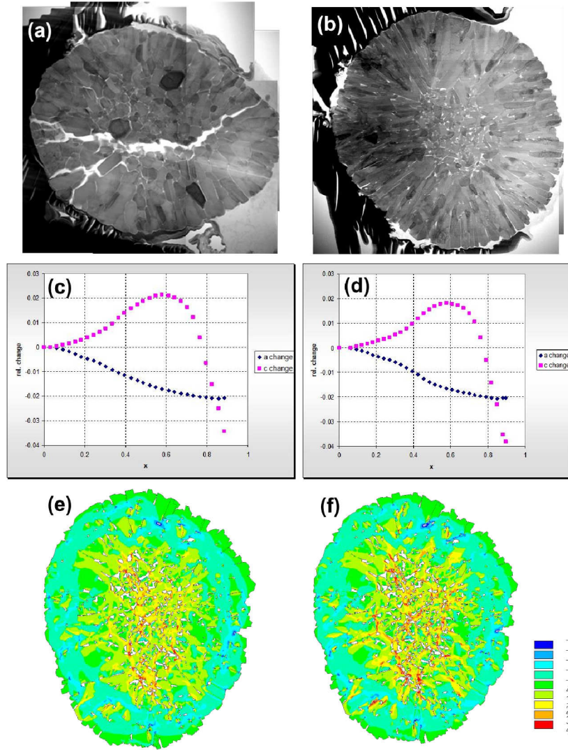
Fig. S1. Cross-sectional TEM image of (a) P-NCA89 and (b) B-NCA88. The particles in panel (a) and (b) are fully discharged state after 100 cycles using coin-type half-cells. Anisotropic lattice parameters change of (c) P-NCA-89 and (d) B-NCA-88 as function of the state of charge ( x ) measured by XRD. The change along the b axis equals the change along the a axis. Calculated stress distribution (maximum principal stress S_{max} in MPa) at x=0.6 in B-NCA-88 particle using (e) isotropic stiffness data of NMC532 reported by Xu et al [21]. and (f) anisotropic stiffness matrix of \text{Li}_{0.5}\text{CoO}_2 from Yamakawa et al [20].
