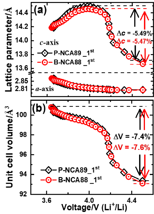
Fig. 5. Variation in (a) a -axis and c -axis lattice parameters and (b) unit cell volume as a function of voltage.
