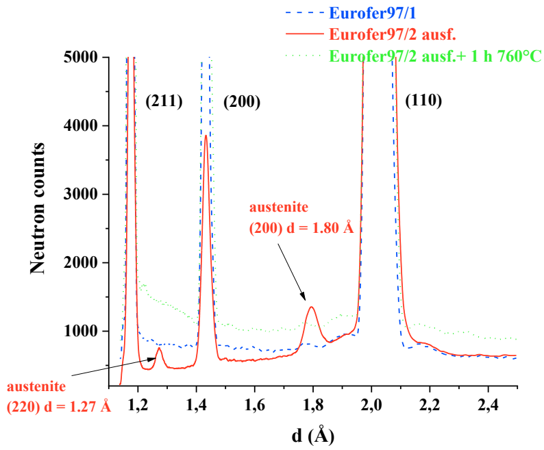
Fig. 7 - Neutron diffractograms (normalized neutron counts vs lattice plane distance, in Å) for the same samples of fig. 3: Eurofer97/1 reference heat 83697, 1040 °C 30' + 750° C 1.5 h (blue, dashed line), Eurofer97/2 1175 °C 30' + ausformed at 650° C (red, continuous line) and Eurofer97/2 1175 °C 30' + ausformed at 650° C + 1 h C 760°C (green, dotted line). Due to the low instrument resolution at 2.1 Å [20], the (111) austenite and (110) Eurofer peaks could not be separated.
